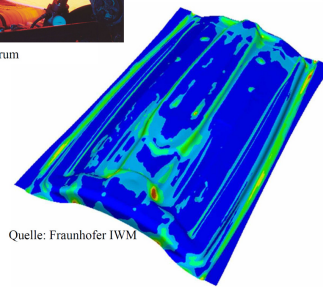
Abb.: Process simulation in forming technology: forming processes, continuum mechanics and simulation methods
