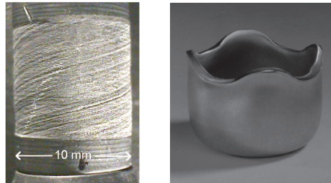
Figure: Plastic Torsion (left); earing with deep drawing (right)
